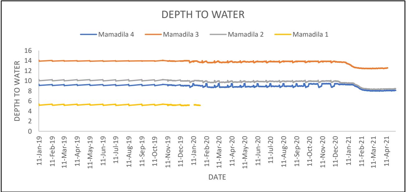
Elevation, Total head and depth-to-water plots locations in mamadila (1-4) between January 2020 to April 2021
